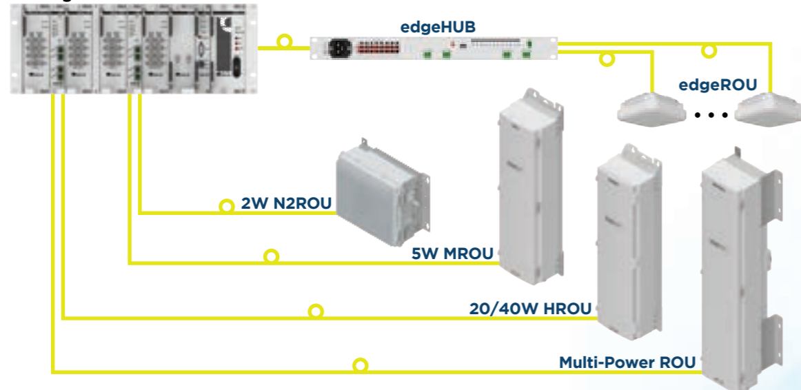
iBIU Signal Interface
