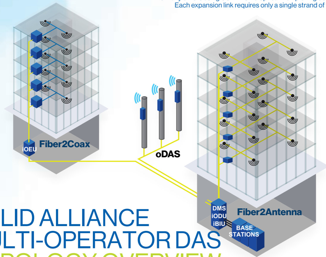
DMS1200 System Management
